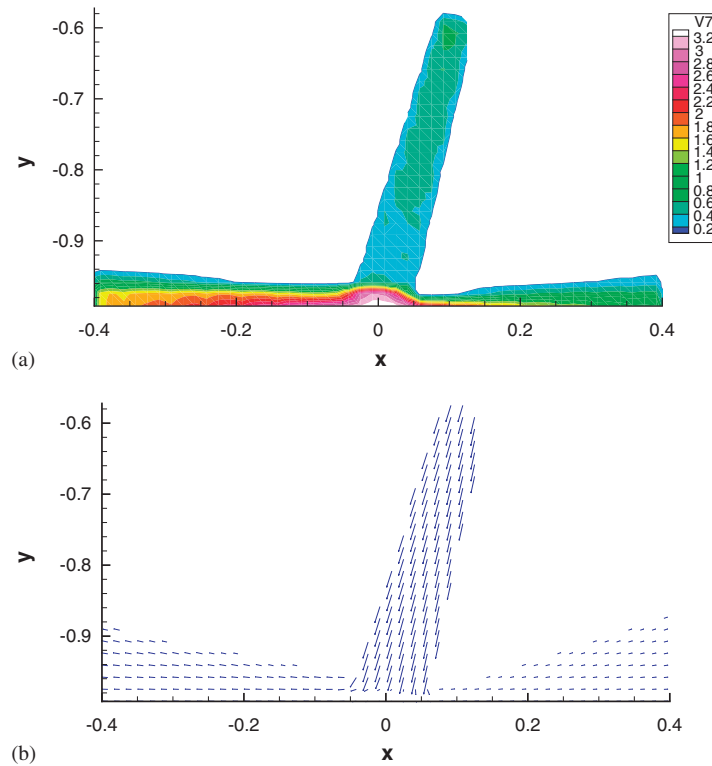
Figure 4. Time and volume averaged: (a) density and (b) velocity.
