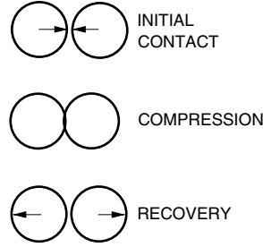
Fig. 1. Compression and recovery of two impacting particles.
